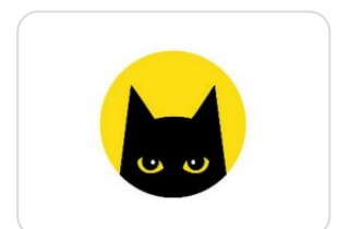
ALICE & BOB
